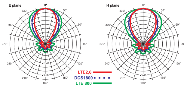
Radiation pattern of antenna: LAT - 56
